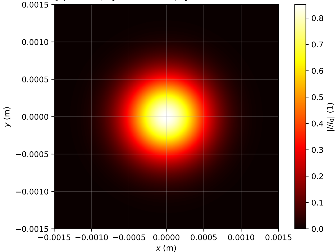
Intensity profile I(x, y, z = 0.955m)/I_0 , Pin=0.1Pcr, artificial time
